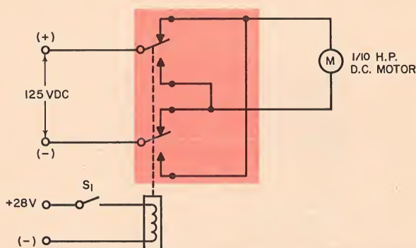
Parallel-opposition arrangement of relay contacts reverses a dc motor.
