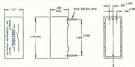
RELAY SHOWN: SPST NORMALLY OPEN (A)
