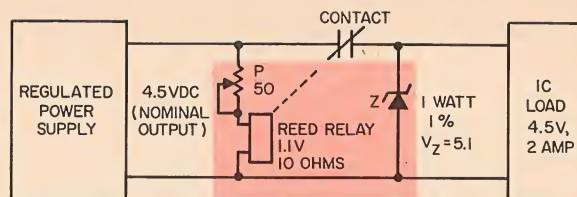
Combination reed relay and zener diode protect an integrated circuit from overvoltage.
