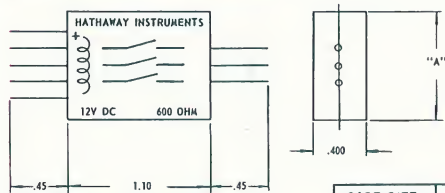
RELAY SHOWN: 3 PST NORMALLY OPEN (A)
